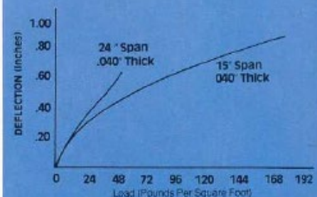
TRANSVERSE LOAD DEFLECTION
